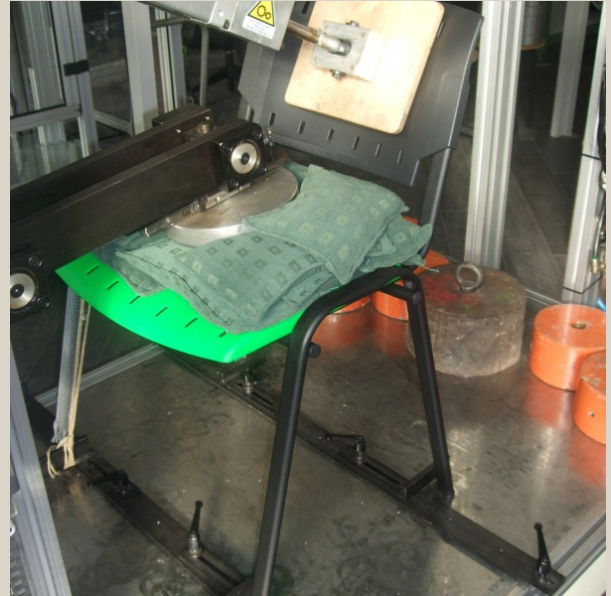
Static load test 1 st level
