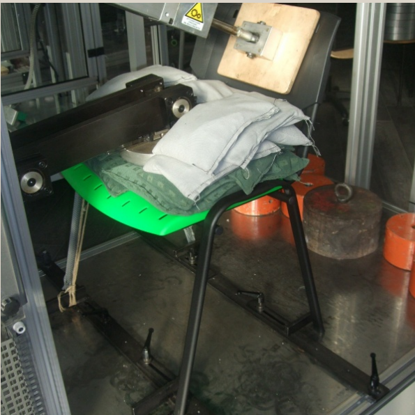
Static load test 2 nd level
