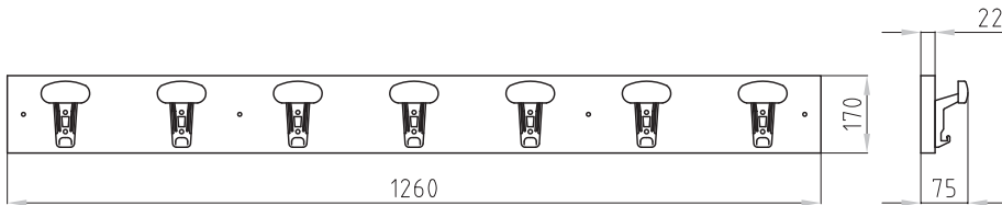
Art. OM 4.384 Attaccapanni 7 posti Clothes-hook 7 places
