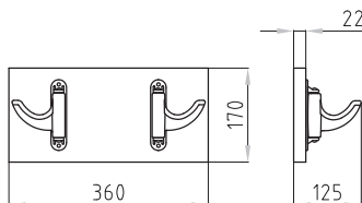
Art. OM 4.388 Attaccapanni 2 posti Clothes-hook 2 places
